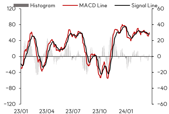
나스닥 MACD
